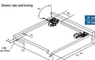
Drawer size and boring
