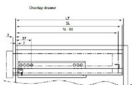
Installation dimensions
