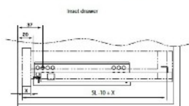
Installation dimensions
